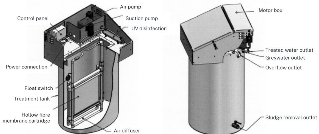
Figure 5-9: Typical Schematic of a GTS
