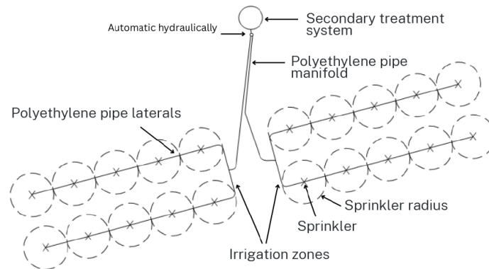
Figure 5-20: Typical Schematic of a Surface Irrigation System
