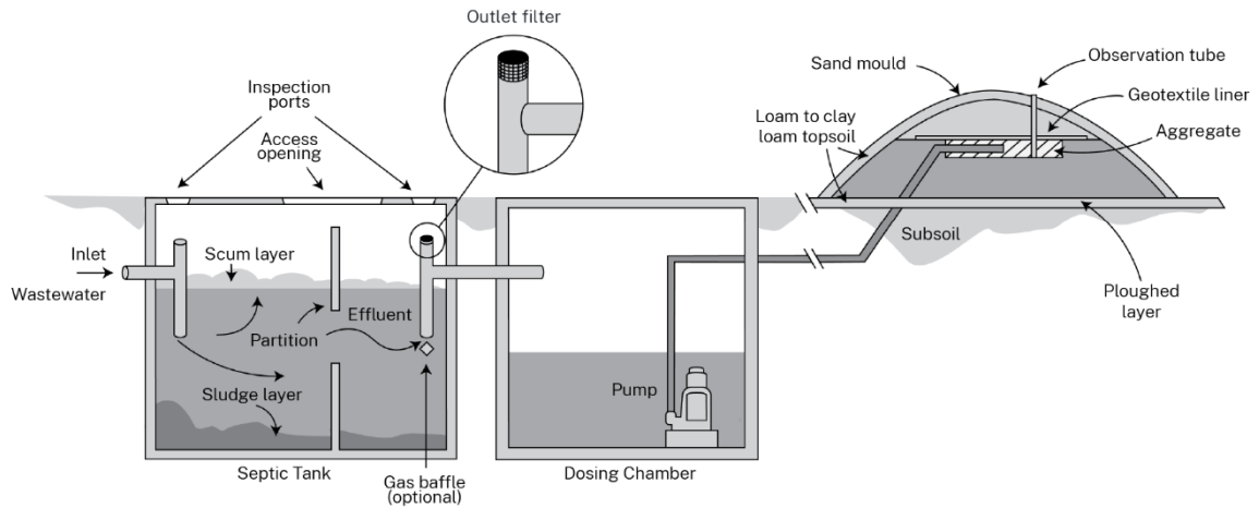
Figure 5-10: Typical Schematic of a Mound System
