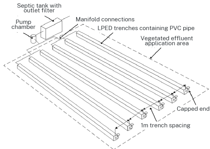
Figure 5-18: Typical Schematic of an LPED System
