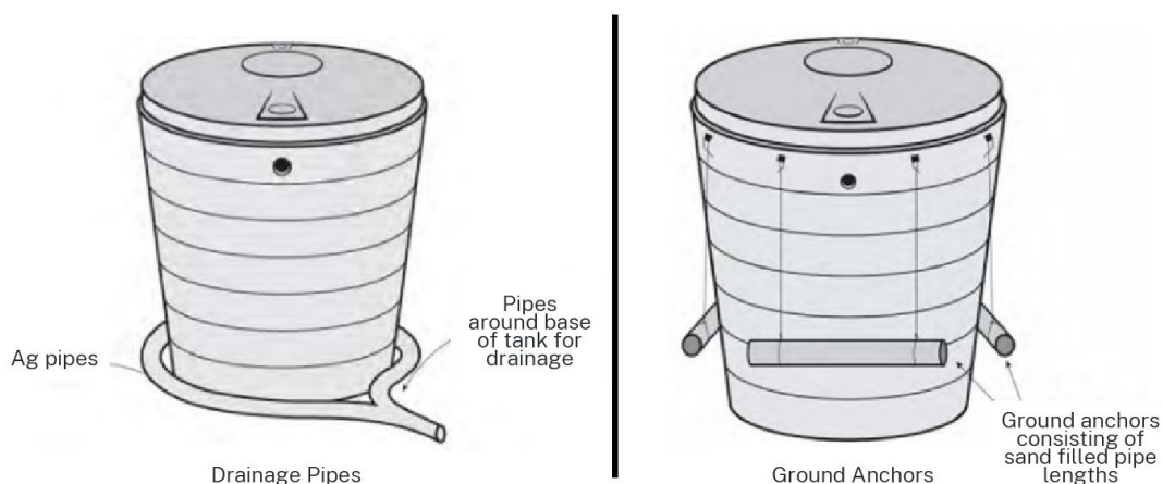
Figure A4-1: Drainage pipes and ground anchors
