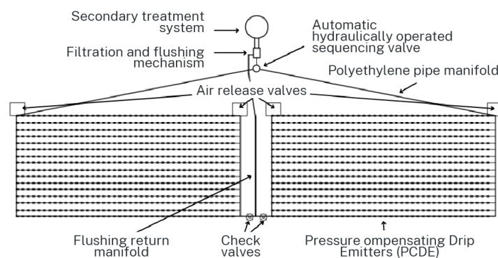
Figure 5-19: Typical Schematic of a Subsurface Irrigation System
