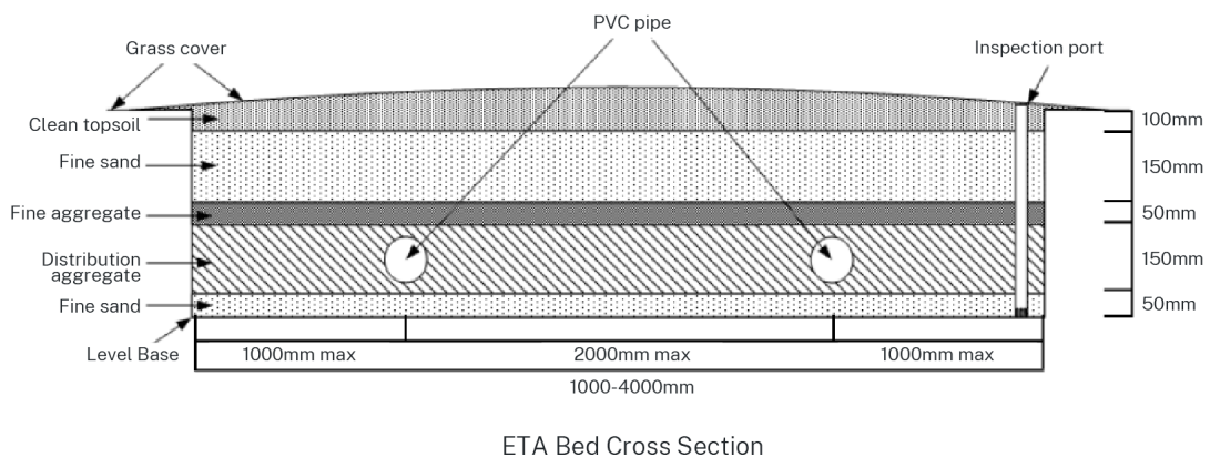
Figure 5-16: Typical Schematic of an ETA Bed
