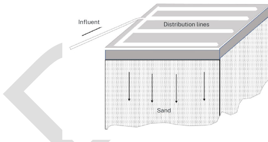
Figure 5-11: Typical Schematic of a Bottomless (Unlined) Sand Filter
