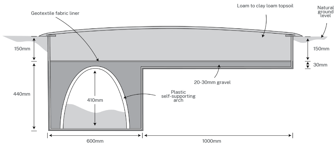
Figure 5-17: Typical Schematic of a Wick System
